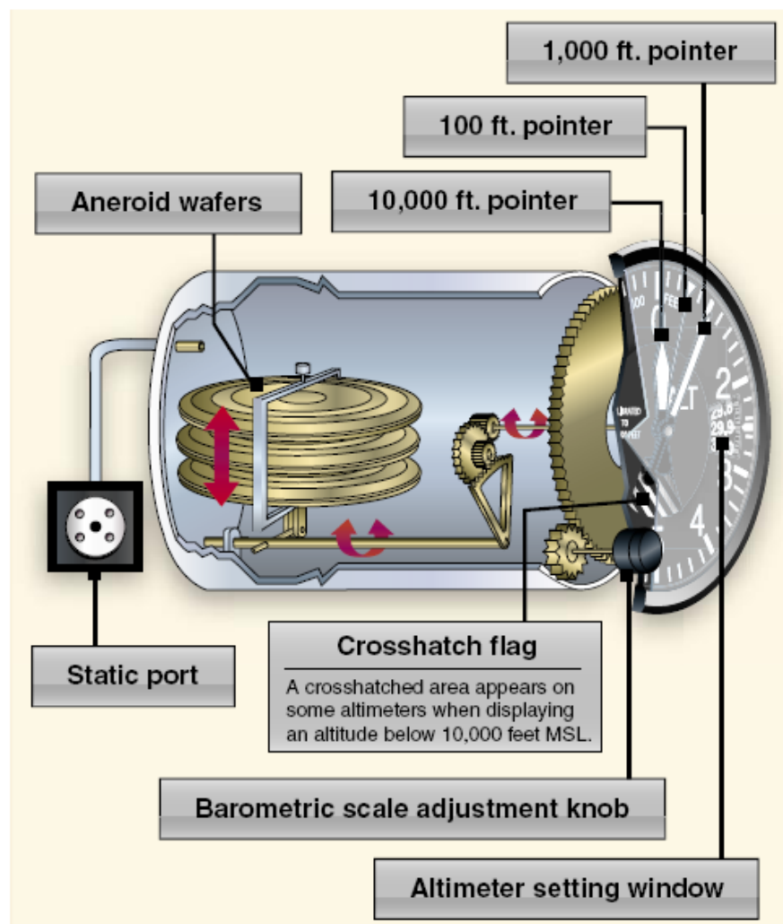
Figure 7-2. Altimeter.
