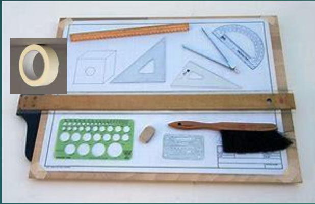
Figure Drawing Board
