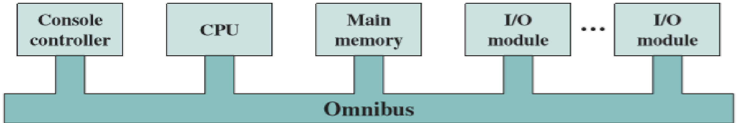
Fig. 6: PDP-8 Bus Structure
