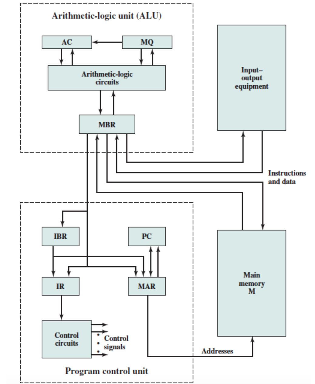
Fig. 2: Expanded Structure of IAS Computer
