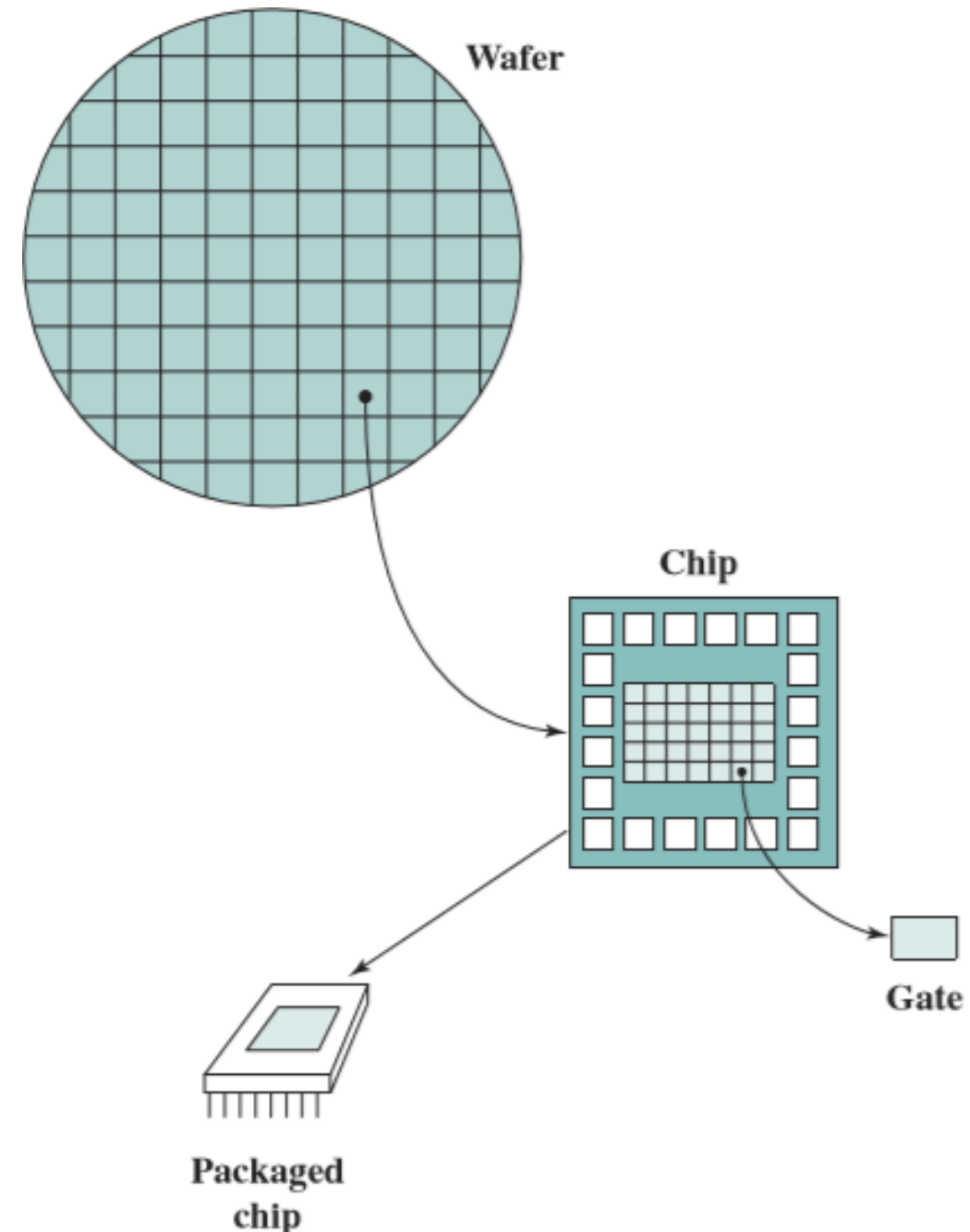
Figure 4: Relation between wafer, chip and gate 37
