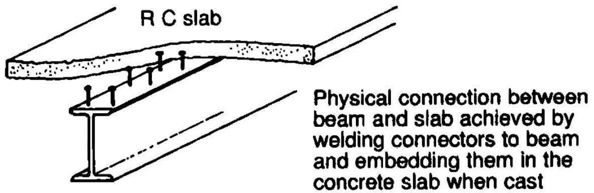
Figure C2.4 Steel beam and RC slab connection
