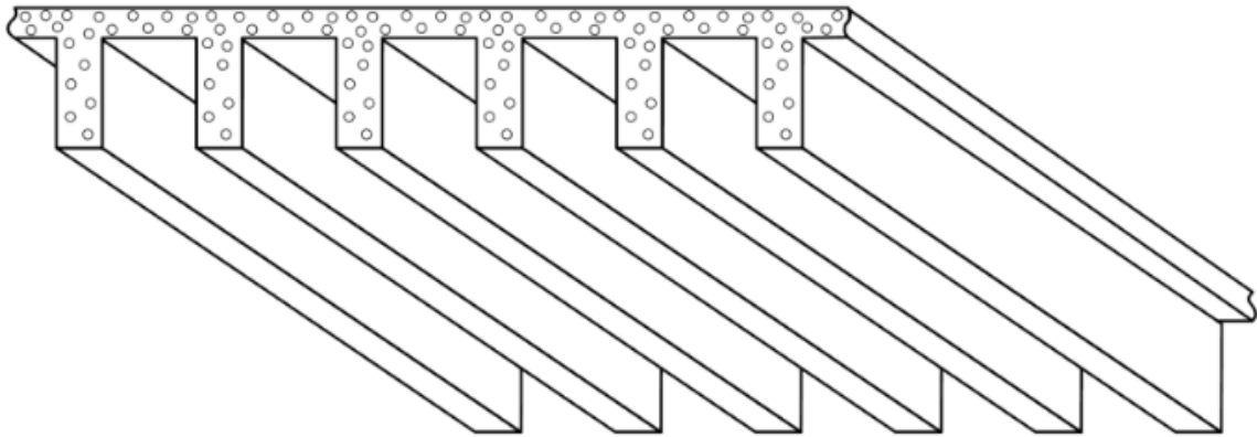
Figure C2.1 suspended concrete slab
