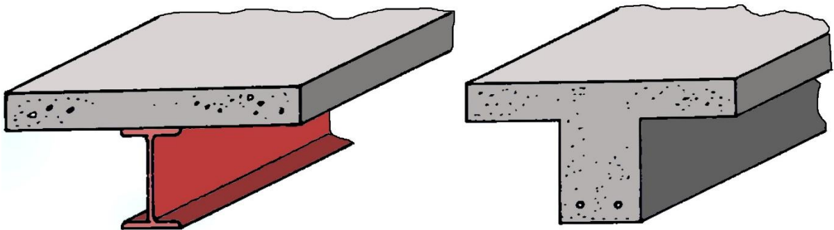
Figure C2.2 Composite beam (left) compared to Reinforced Concrete, RC, beam (right)
