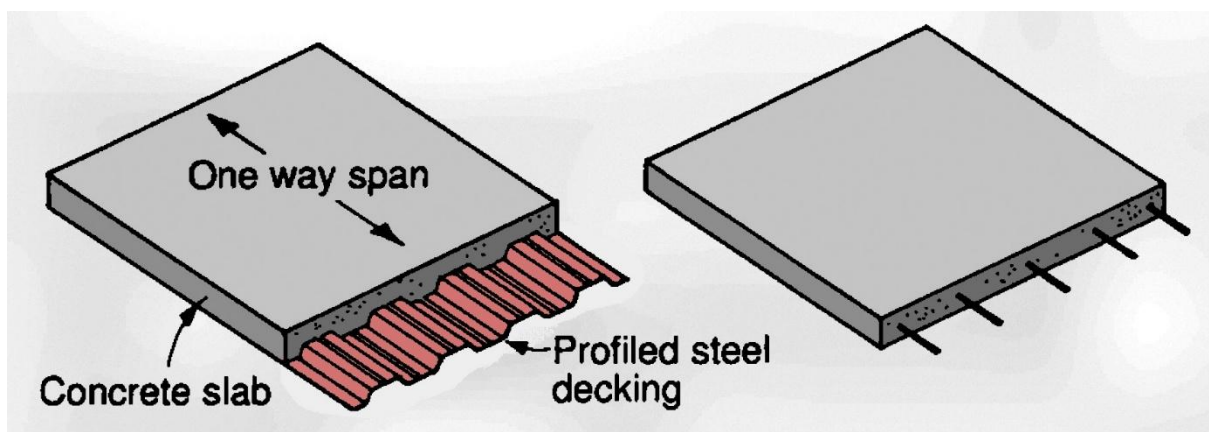
Figure C2.3 composite floor (left) compared to RC floor (right)
