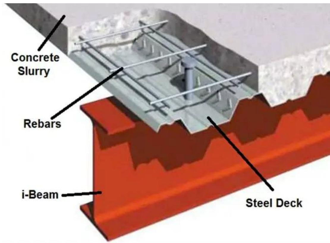
Figure C2.5 Details for composite beam and floor system.
