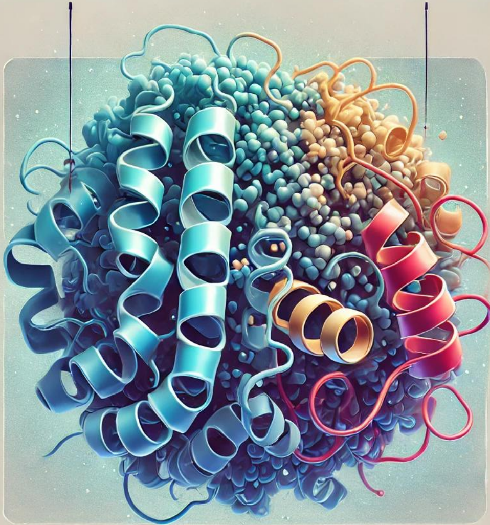
Apoenzyme
